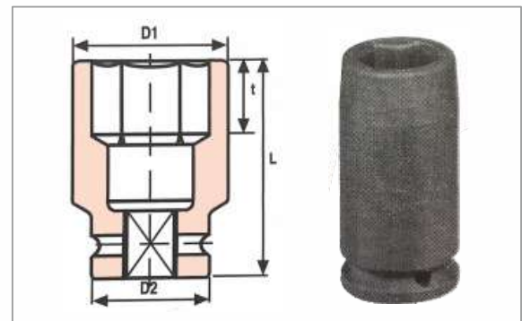
6 POINT IMPACT SOCKETS LONG
