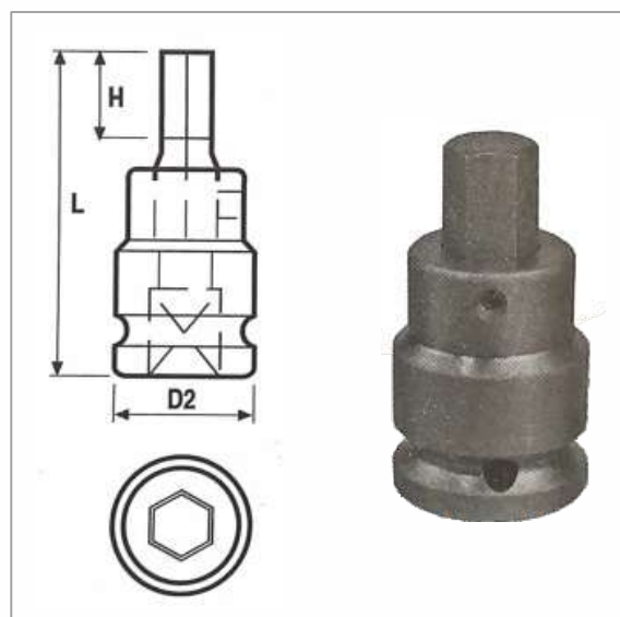
TWO PART INHEX DRIVER
