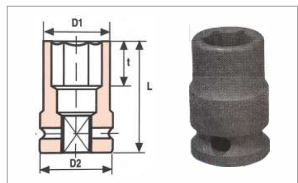
6 POINT THIN WALL IMPACT SOCKETS REGULAR LENGTH
