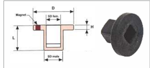
INSERT ADAPTER
