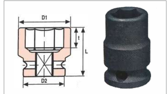
6 POINT IMPACT SOCKETS REGULAR LENGTH
