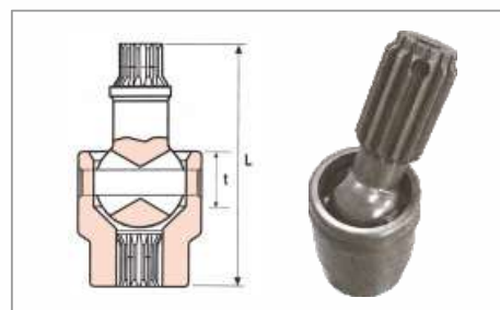
UNIVERSAL JOINT
