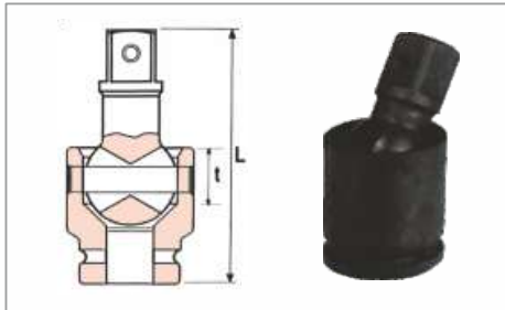
UNIVERSAL JOINT
