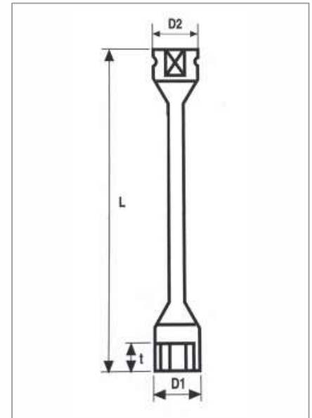
TORSION BARS
