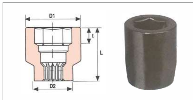
6 POINT IMPACT SOCKETS REGULAR LENGTH
