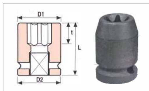
IMPACT SOCKETS FOR TORX® FASTENER
