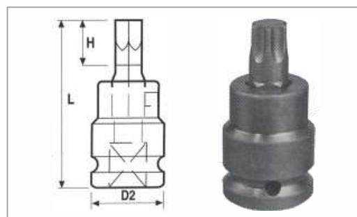
2 PARTS DRIVERS FOR TORX® SCREW
