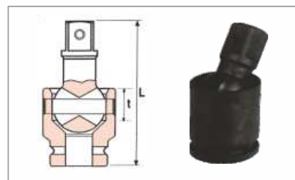
UNIVERSAL JOINT
